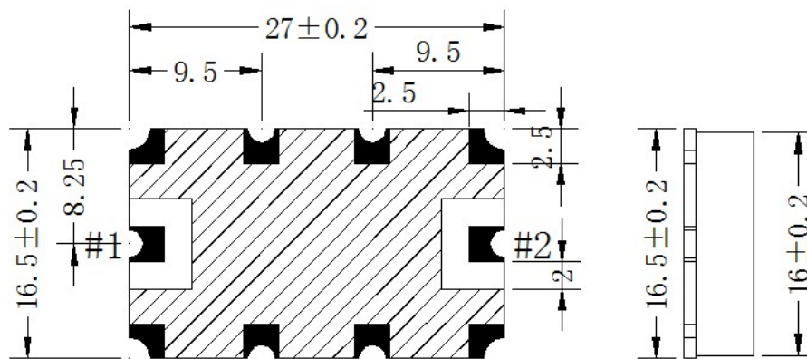
Bottom View
